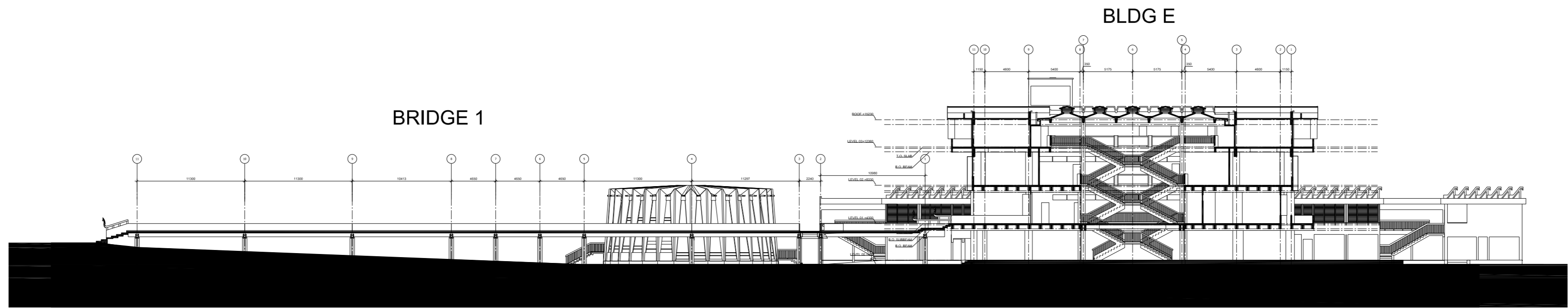
SECTION "AA" SCALE 1/350
