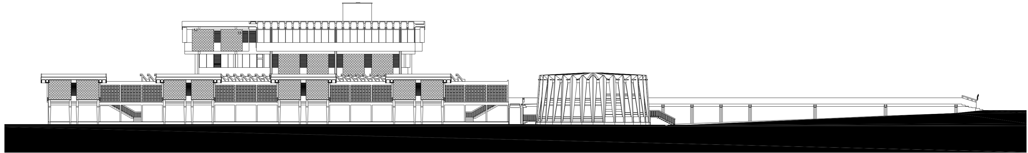
WEST ELEVATION SCALE 1/350
